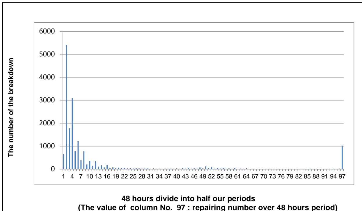
Figure 5: Histogram of the relative frequency of time needed to troubleshoot the unexpected breakdowns of printing machines (Examination period: 1. January, 1988 – 31. December, 2004)
